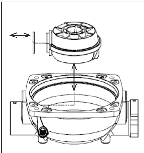
Nutating disc (removal / replacement)
